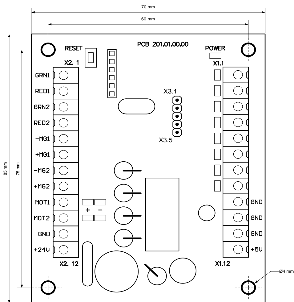
Figure 4 – Appearance of the controller PCB.201.01.00.00
