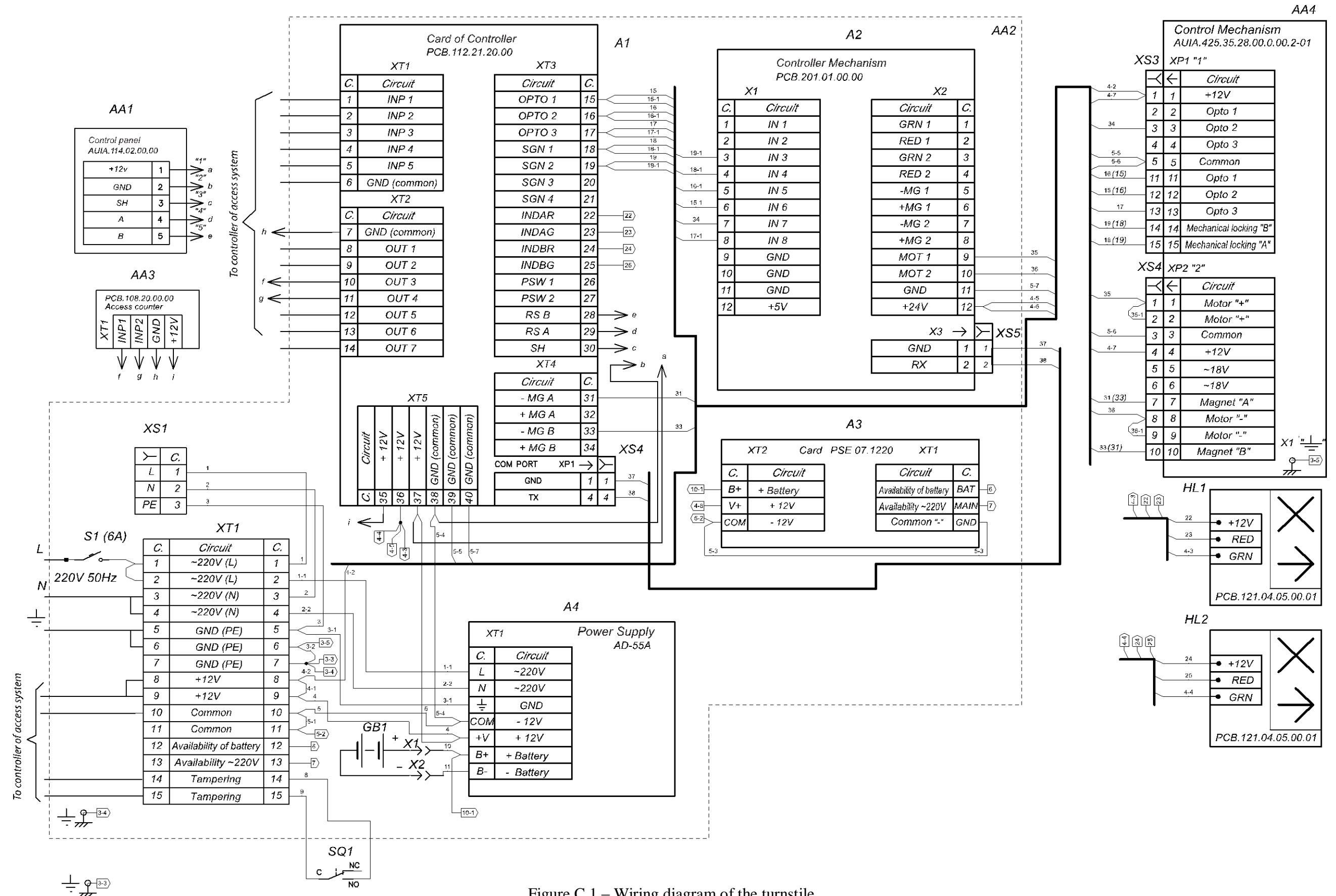
Figure C.1 – Wiring diagram of the turnstile
