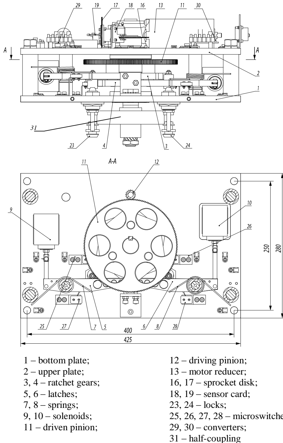
Figure 1 – Control mechanism
